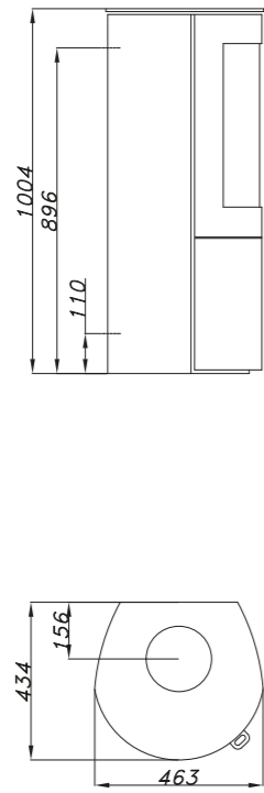
WESTFIRE.UNIQ.26 WEIGHT: 105 KG
