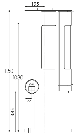
WESTFIRE.UNIQ.36 WESTFIRE.UNIQ.37 PEDESTAL 1 / WEIGHT: 95 KG
