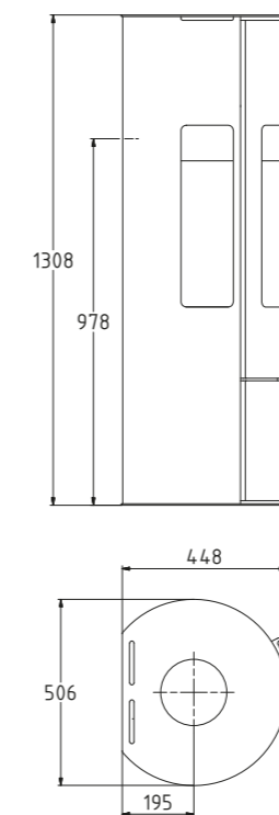
WESTFIRE.UNIQ.37 / LARGE WEIGHT: 110 KG
