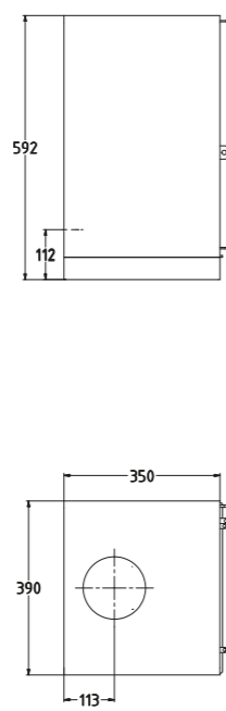
WESTFIRE.UNIQ.35 / 50 MM BLOCK WEIGHT: 95 KG
