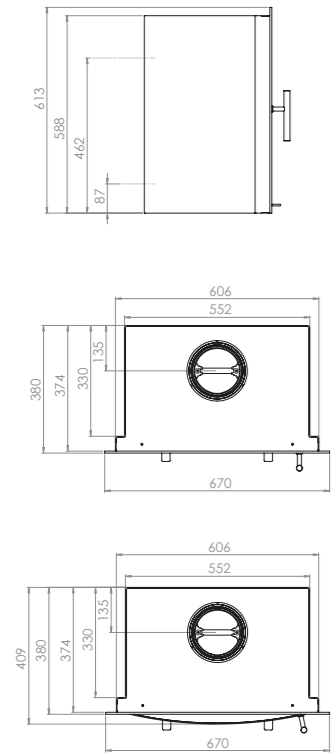
WESTFIRE.UNIQ.23 INSERT 3-SIDED FRAME FLAT / CURVED DOOR WEIGHT: 92 KG
