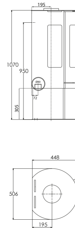
WESTFIRE.UNIQ.36 WESTFIRE.UNIQ.37 PEDESTAL 2 / WEIGHT: 95 KG
