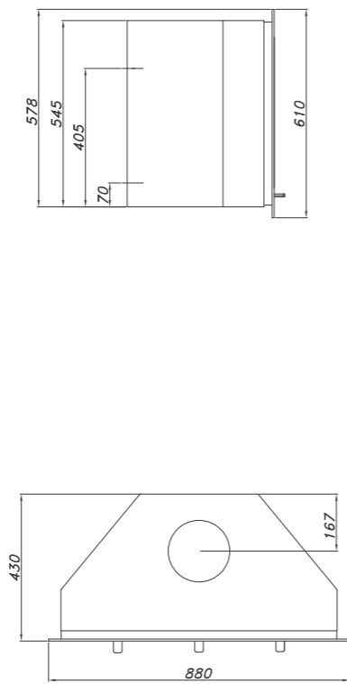
WESTFIRE.UNIQ.32 / INSERT NARROW 4-SIDED FRAME WEIGHT: 110 KG
