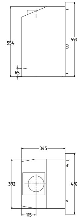
WESTFIRE.UNIQ.35 / INSERT 3-SIDED FRAME WEIGHT: 75 KG
