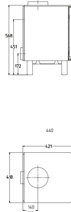
WESTFIRE.ONE WEIGHT: 80 KG
