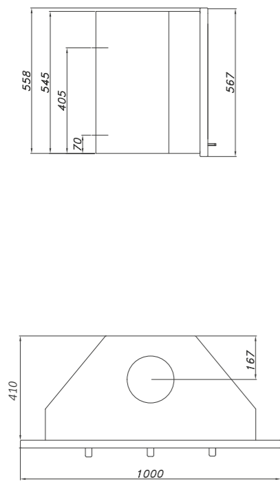
WESTFIRE.UNIQ.32 / INSERT WIDE 4-SIDED FRAME WEIGHT: 110 KG
