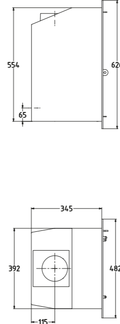
WESTFIRE.UNIQ.35 / INSERT 4-SIDED FRAME WEIGHT: 75 KG
